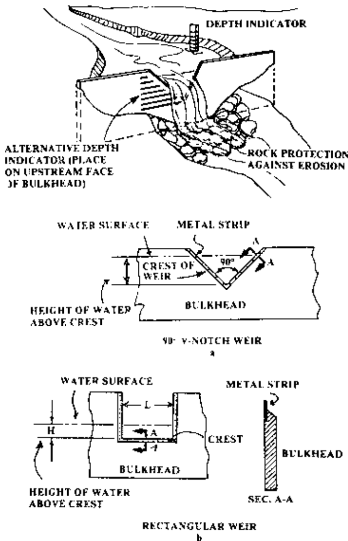
Figure 6.7 - Standard Weirs
