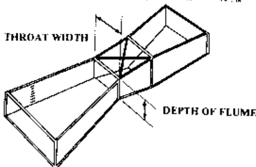
Figure 6.8 Parshall Flume
