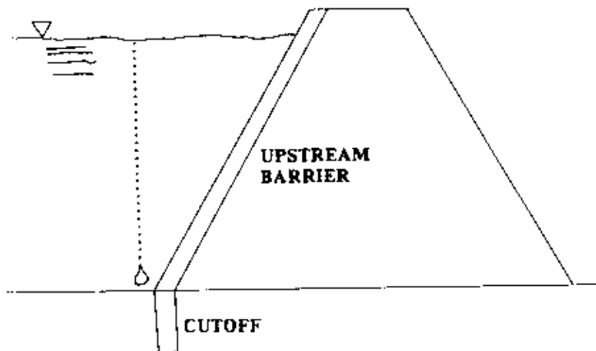
Figure 2.2 Embankment Dam
