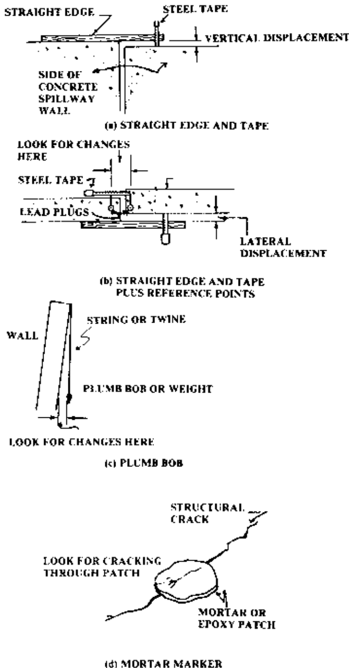
Figure 6.4 - Measuring Displacements
