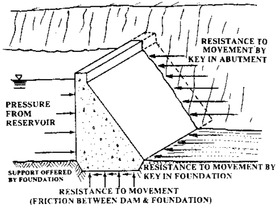
Figure 2.3 Concrete Gravity Dam
